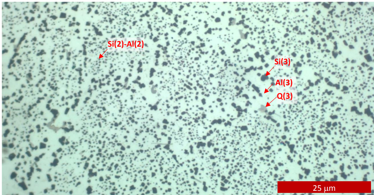
Fig. 2. Typical microstructure of squeeze-cast and heat-treated (Al 20Si 3Cu 0.5Mg 0.5Fe) in-situ formed ultrafine metal matrix composite using unique Universal Metallurgical Simulator and Analyzer Platform. (LOM, HOV = 100 \mu m), [1, 7].
