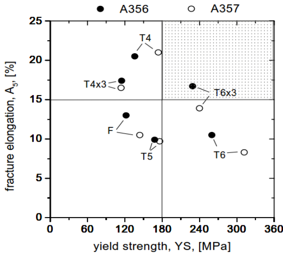
Fig. 4. Dependence of fracture elongation and YS on heat treatment for thixocast A356 and A357 alloys. Note little change in elongation between T4x3 and T6x3 that share the short 3 min solution and spheroidization treatment. Ogris [4]
