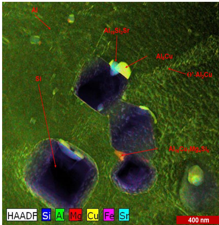
Fig. 3. Squeeze-cast and heat-treated (Al 20Si 3Cu 0.5Mg 0.5Fe) in-situ formed ultrafine metal matrix composite. (HAADF-STEM, HOV = 2 μm), [1].
