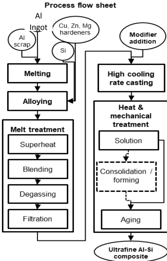
Figure 4: Composite production process schematic
