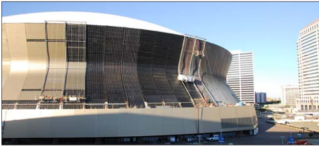
Figure 2. Installation of the anodized aluminum panels has begun on the exterior of the Louisiana Superdome.
